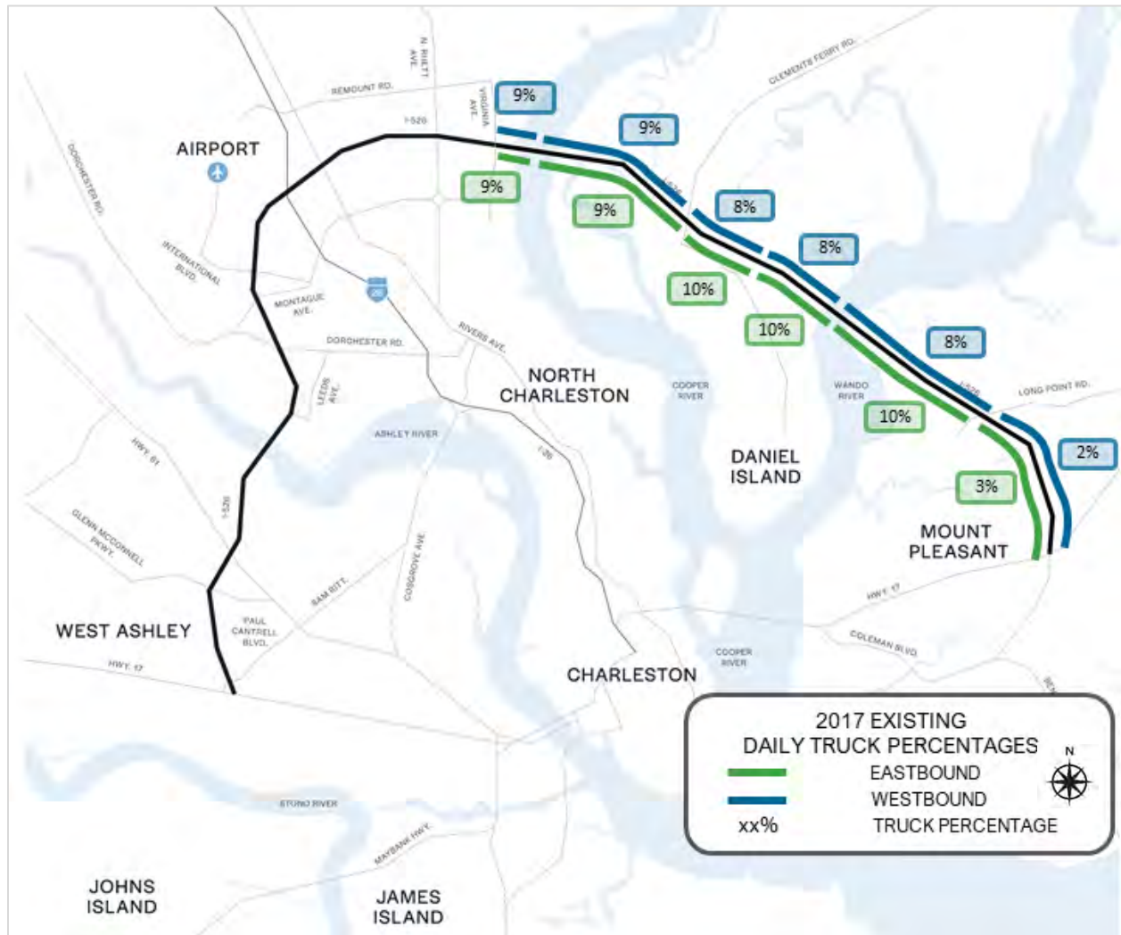
Figure 2-5: Percent Daily Trucks by Segment (2017)
